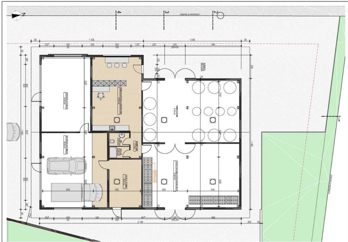
PIANTA PIANO TERRA - ±0.00
